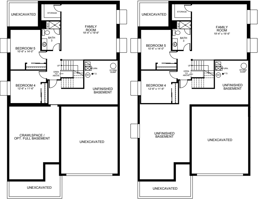
PARTIAL FINISHED BASEMENT
