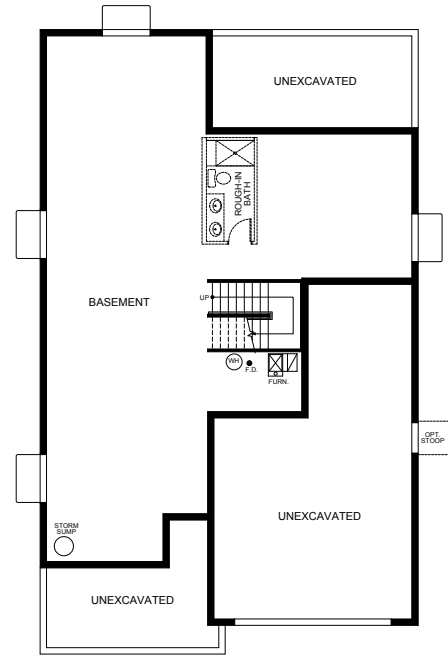
UNFINISHED FULL BASEMENT
